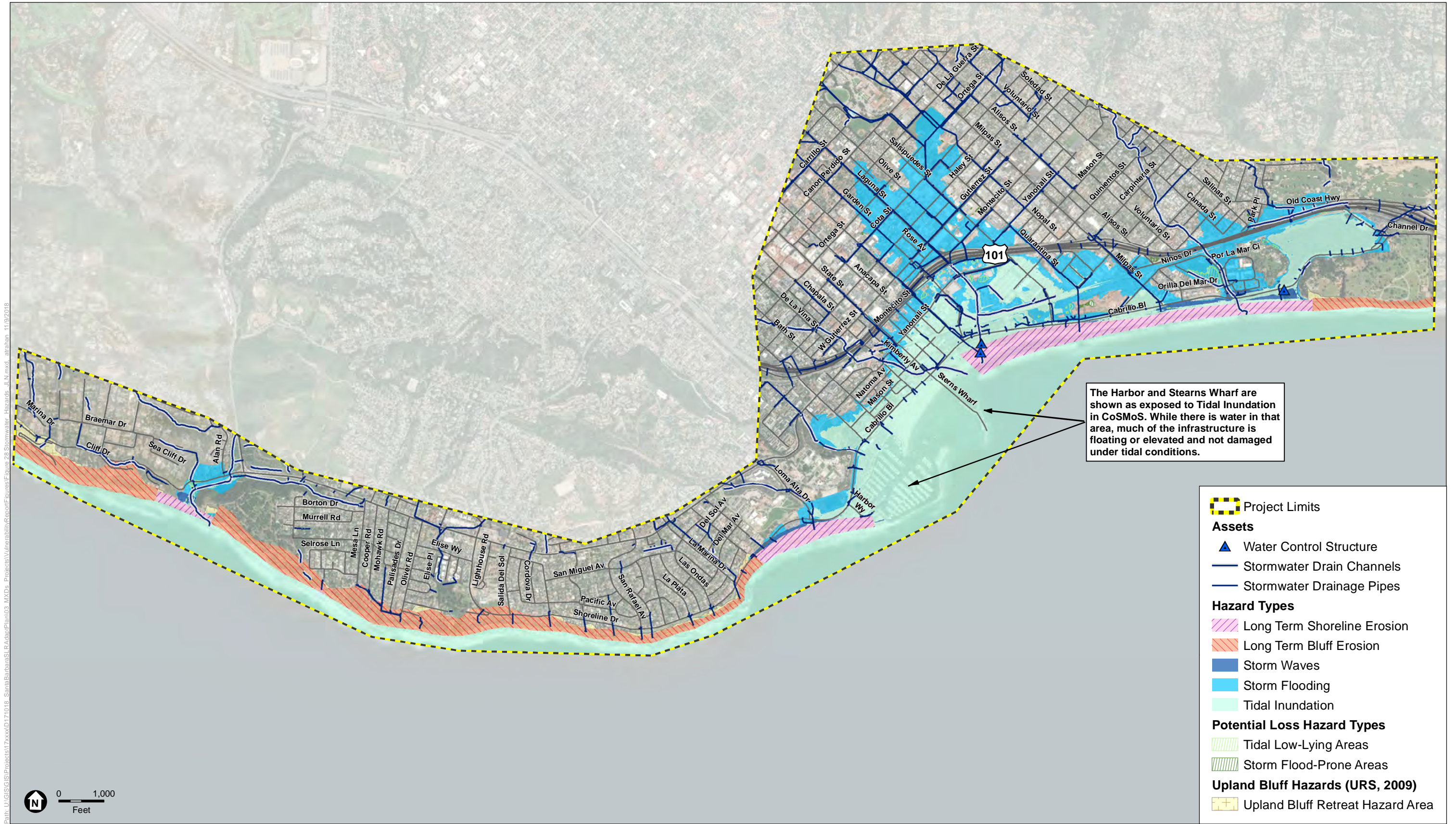
Figure 28 Asset Hazard Map: Stormwater Hazards with 6.6 ft SLR
