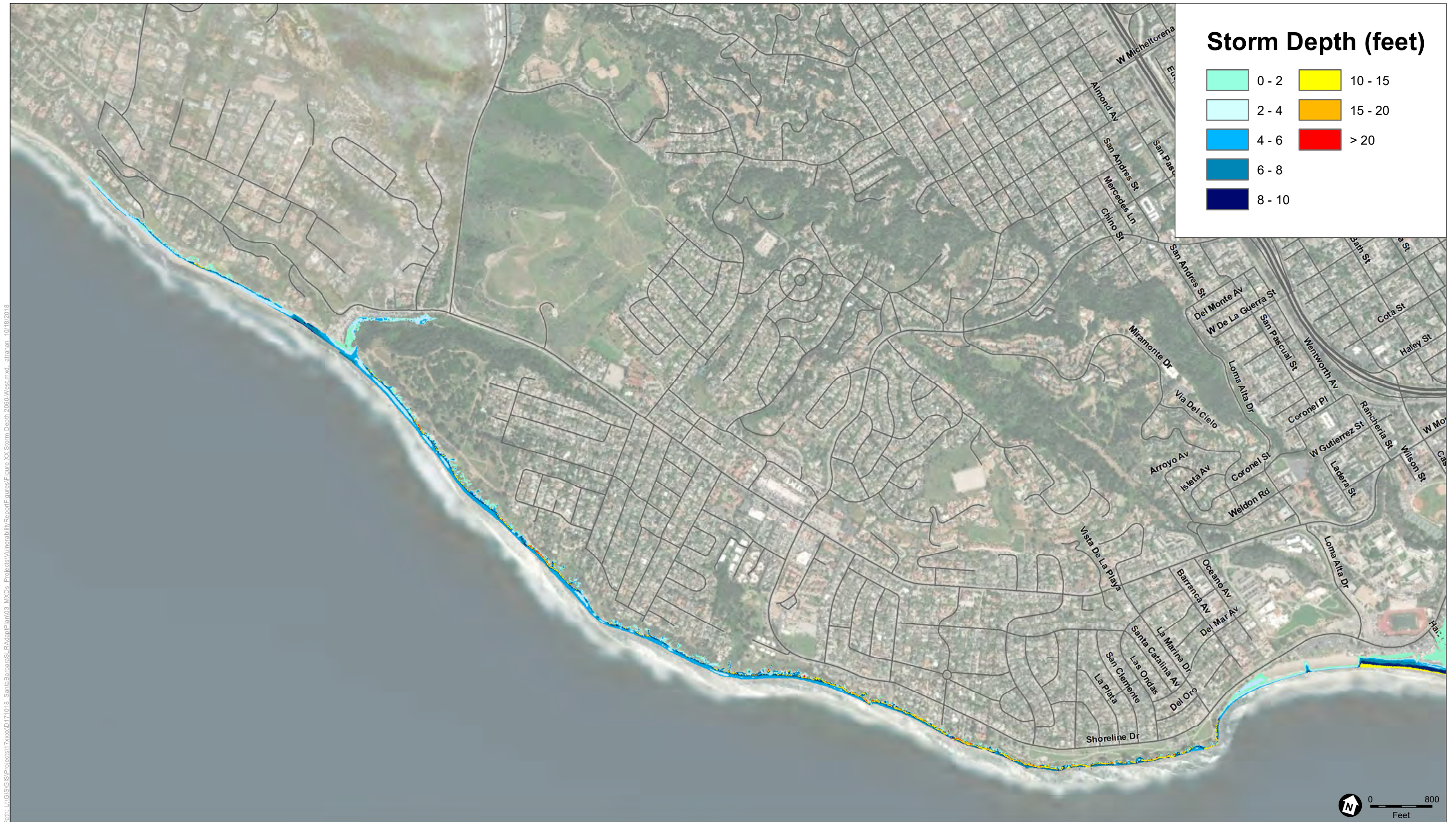
Figure 22 2060 Storm Inundation Depth (West)
