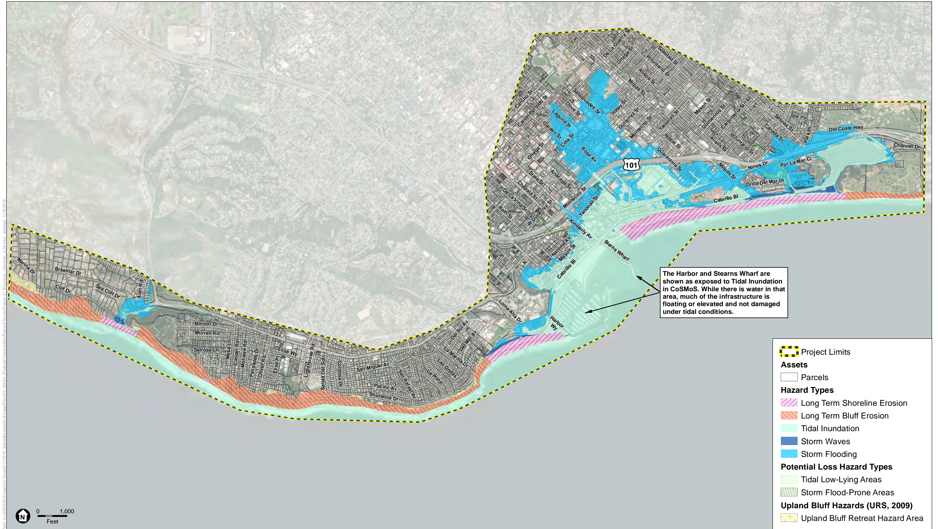
Figure 31 Asset Hazard Map: Public and Private Properties Hazards with 6.6 ft SLR
