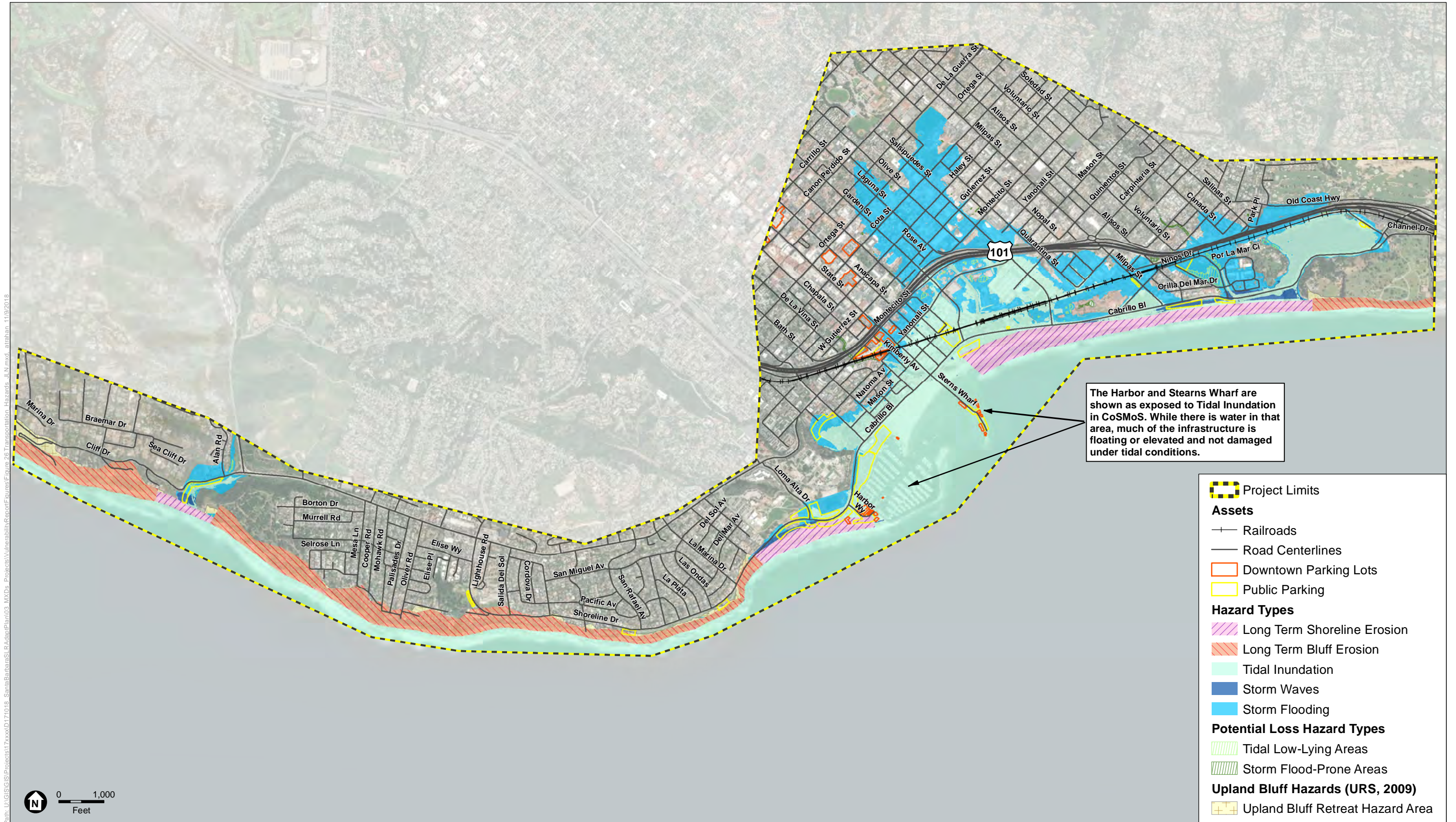
Figure 26 Asset Hazard Map: Transportation Hazards with 6.6 ft SLR
