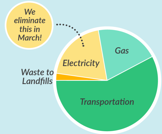
Santa Barbara's Current Carbon Emissions
